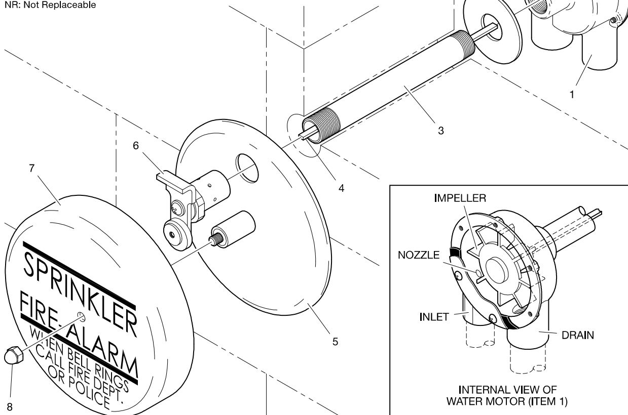
FIGURE 1 MODEL WMA-1 WATER MOTOR ALARM ASSEMBLY
